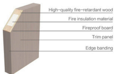
Fire-proof door inside M-07
